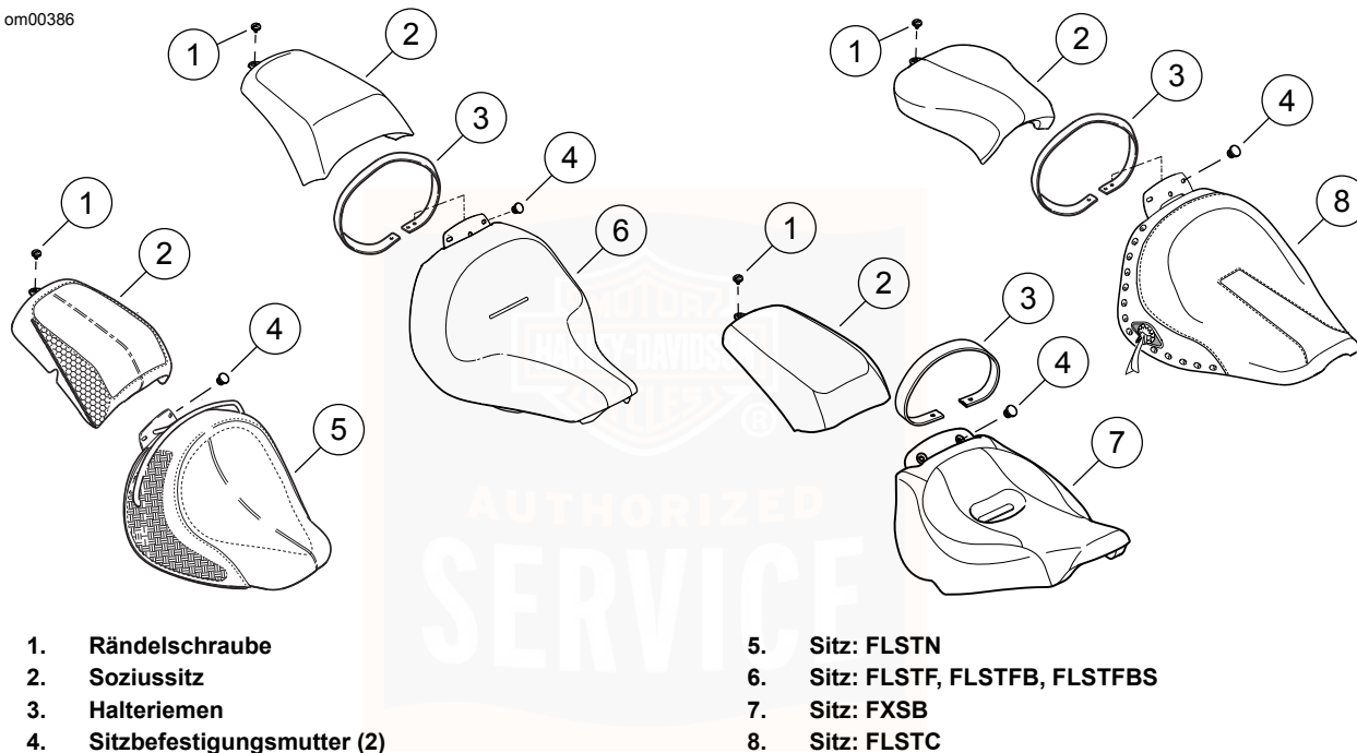
Abbildung 78. Sitz: FLSTC, FLSTF, FLSTFB, FLSTFBS, FLSTN, FXSB
